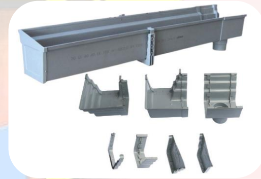
PVC Rain Gutter and Accessories
